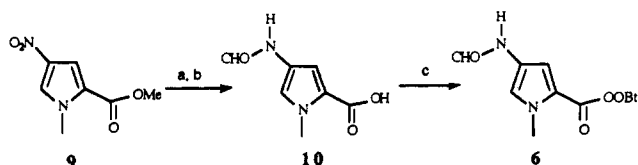
Scheme 5 a
