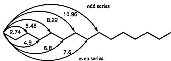
Scheme 4 a
