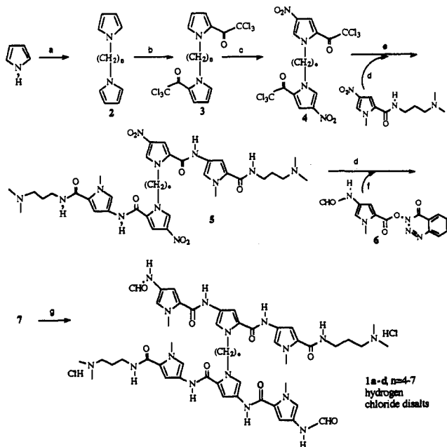
Scheme 4 a
