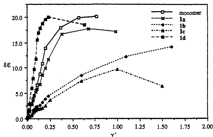
Figure 3. CD titration curves with poly(A-T)-poly(A-T) DNA. The monitoring wavelength is set at 330 nm. For 1c,d , the precipitation of DNA out of solution at the end of the titration was observed. The decrease of \delta\epsilon is obvious from their titration curves.
